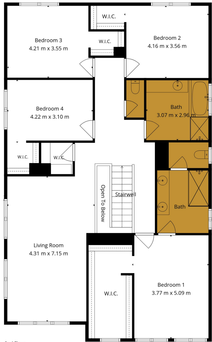
2nd Floor
