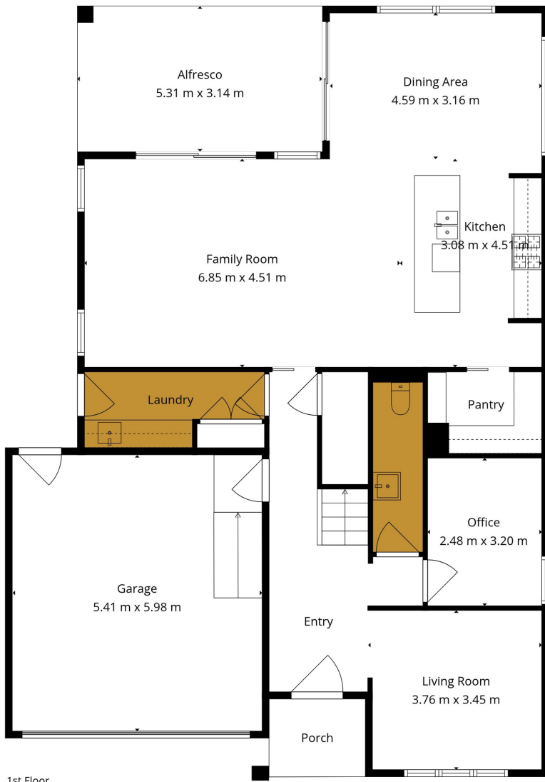
1st Floor
